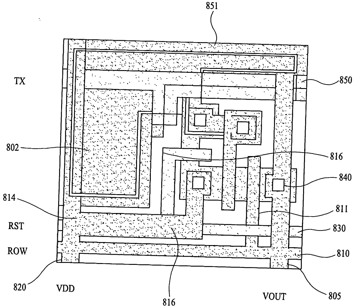
FIG. 7 (PRIOR ART)
